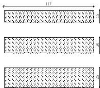
Tile Details
