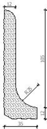
Cove Section
